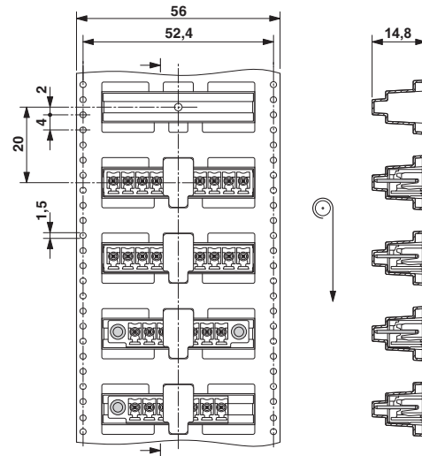
Dimensional drawing
